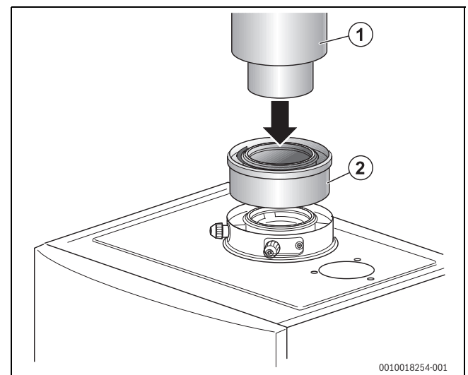
Fig. 4 Concentric pipe (sealed combustion)
