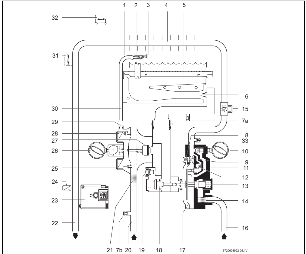
Fig. 2 Functional diagram
