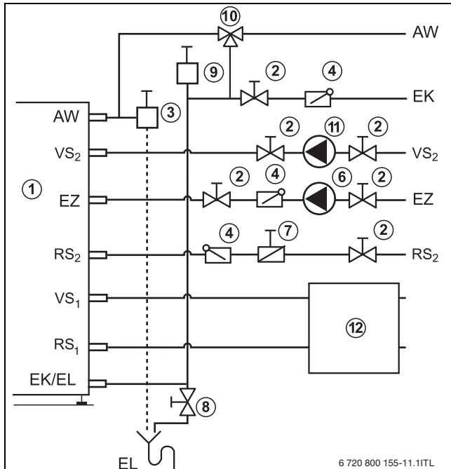
Fig. 12 Installation (illustrative)
