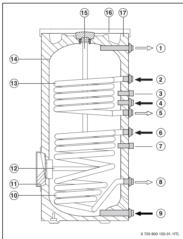
Fig. 2 SM80/5, SM100/5
