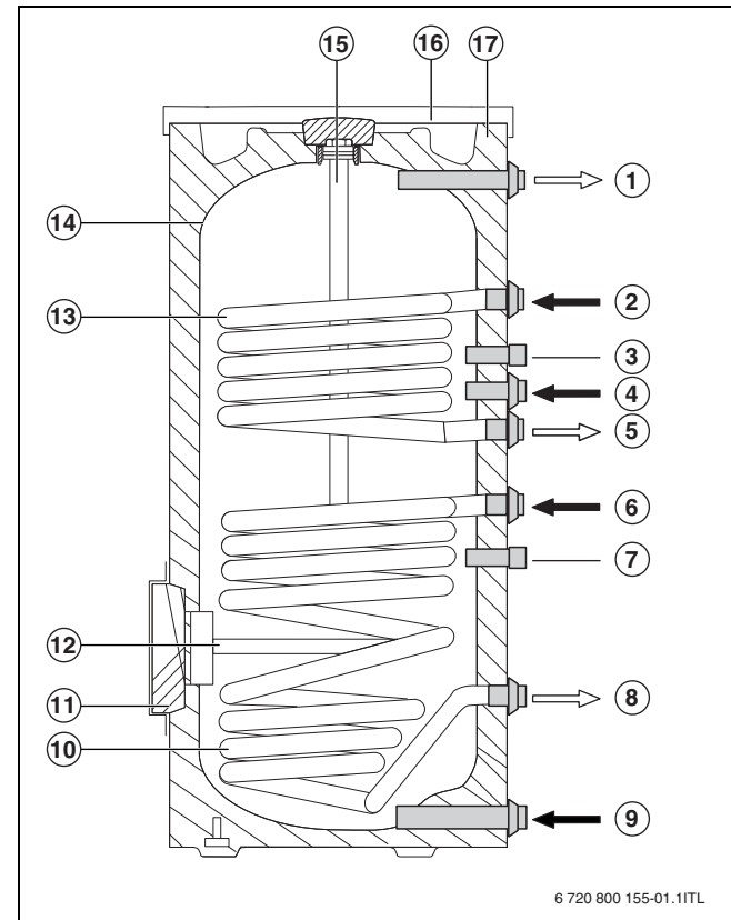
Fig. 2 SM80/5, SM100/5
