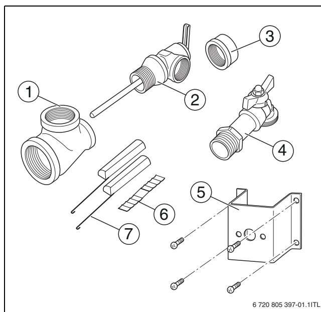
Fig. 1 Tank components
