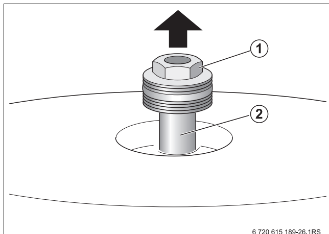
Fig. 21 Checking the top magnesium anode
