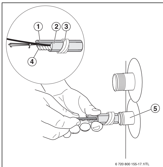
Fig. 14 Installing the DHW temperature sensor
