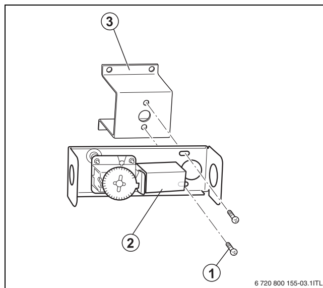
Fig. 16 Screw the bracket onto the aquastat
