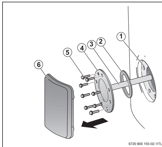
Fig. 23 Reinstall handhole cover
