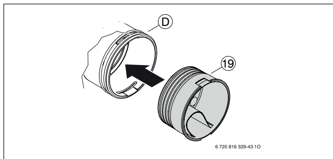
Rys. 116 RR 75... + RRS 75
