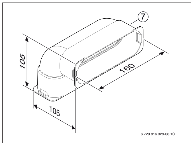
Rys. 120 FKB 140-1 [7] FKB 140-1
