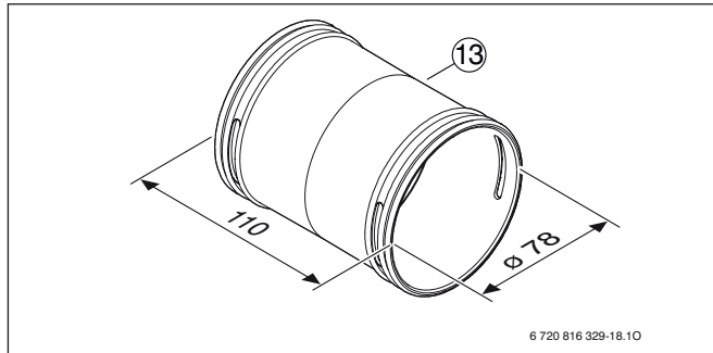
Rys. 114 RRV 75
