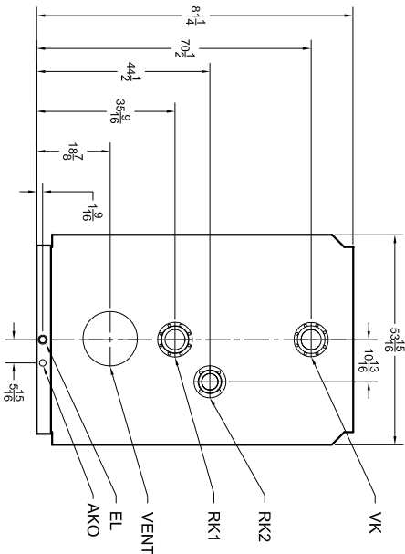
REAR VIEW
