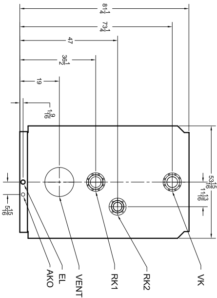
REAR VIEW
