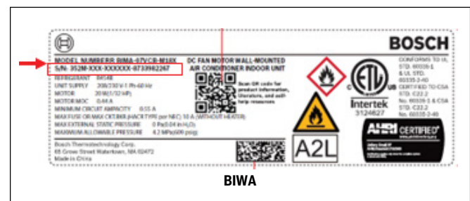
Figure 30 BIWA indoor unit rating plate
