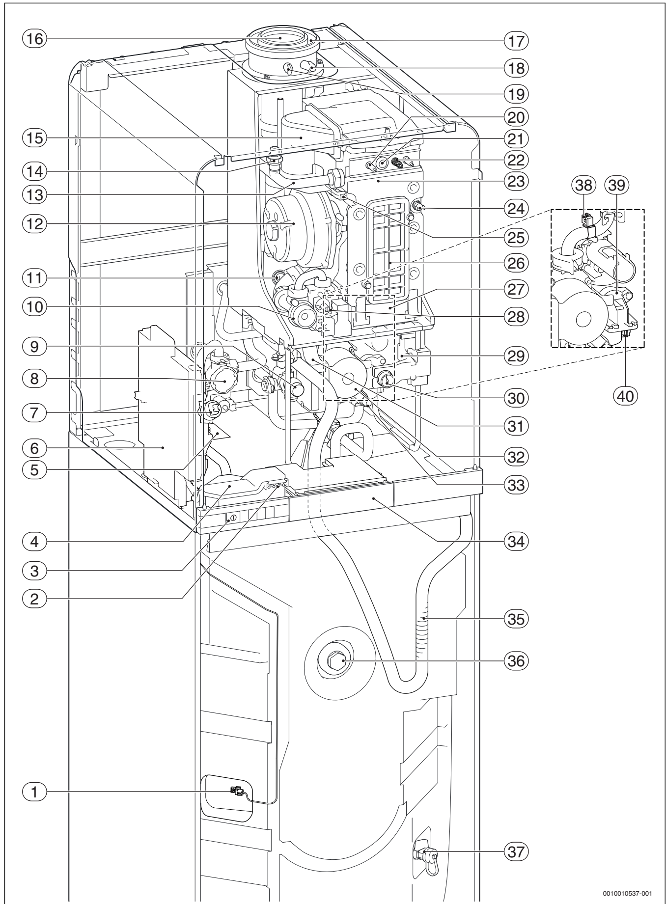
Fig. 17 Chaudières GC9000iWM 30/150
